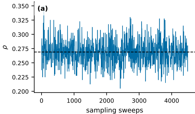
Noninteracting run: \mu = -1
